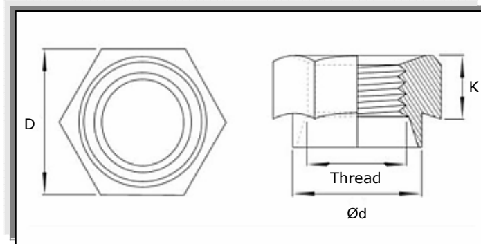
Data sheet for Metric Hexagon Rivet Bushes
