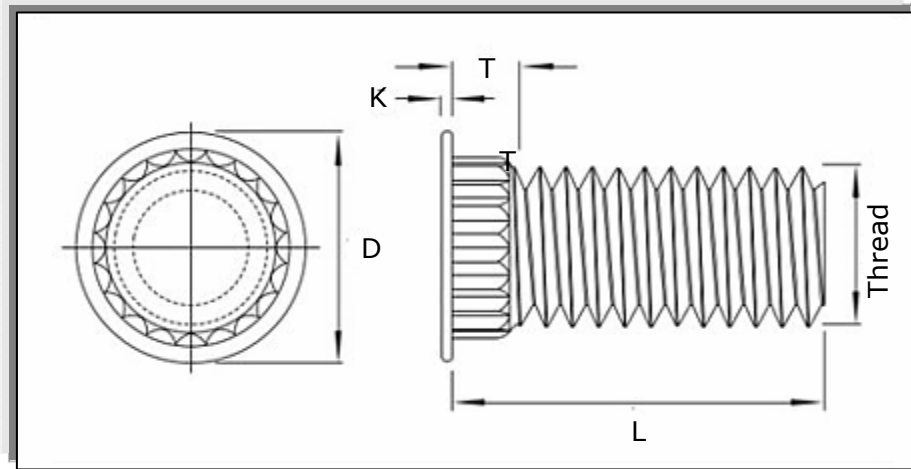
Data sheet for Metric Broaching Studs
